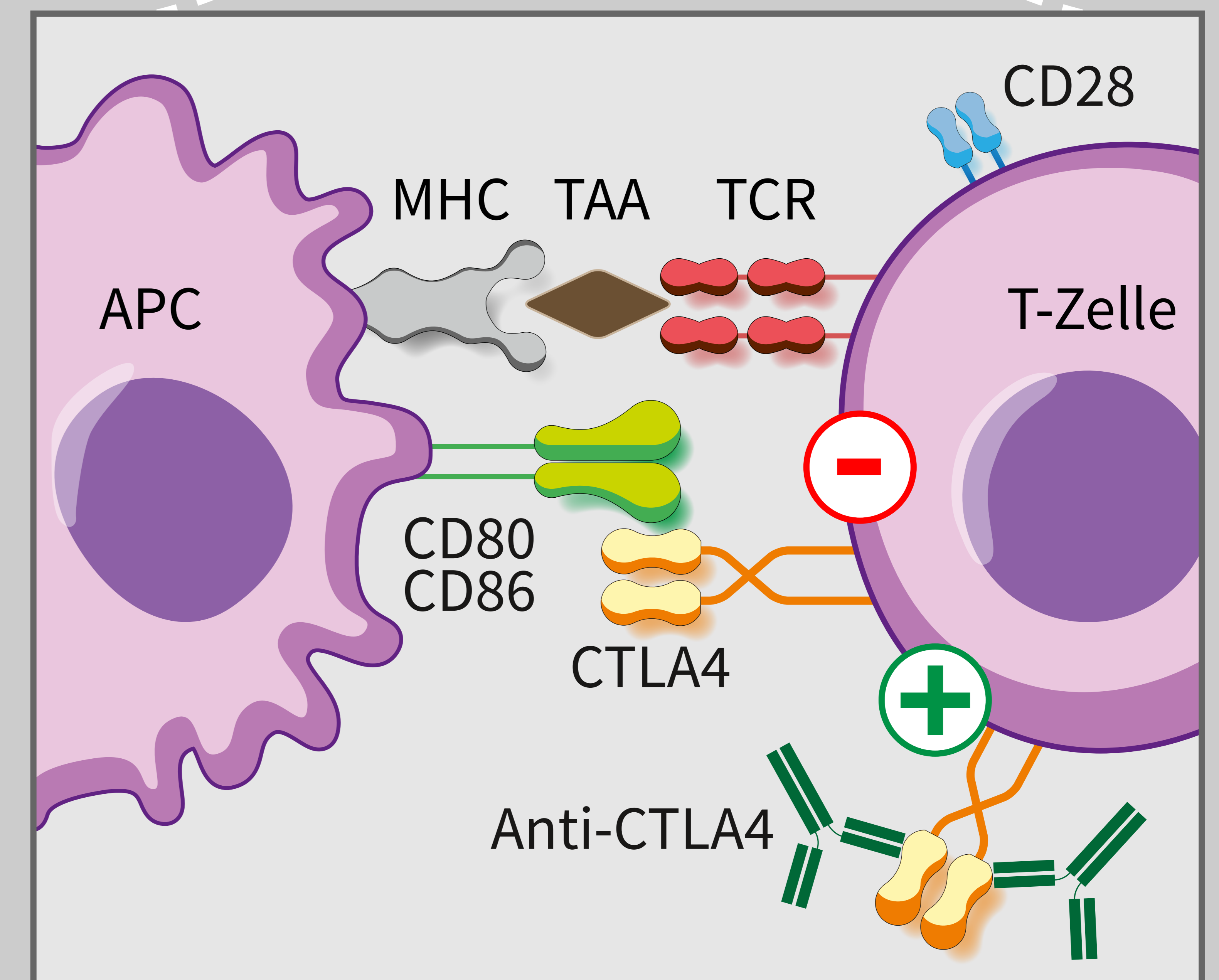
Priming
